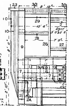
Fig. 412. Half Rear End Elevation.
